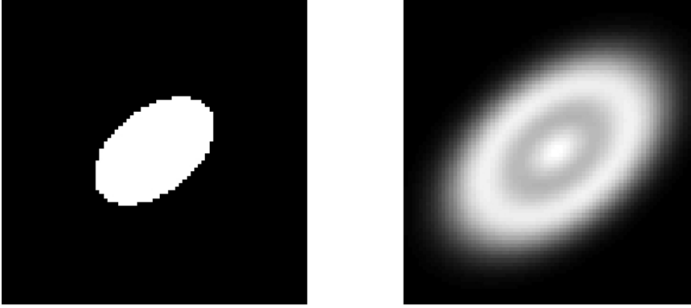
FIGURE 5. Sheared circle f_{0.5} (left) and \mathbb{T}_{(\psi_2, 1, 0.5)} (right, "matching" shear factor).
