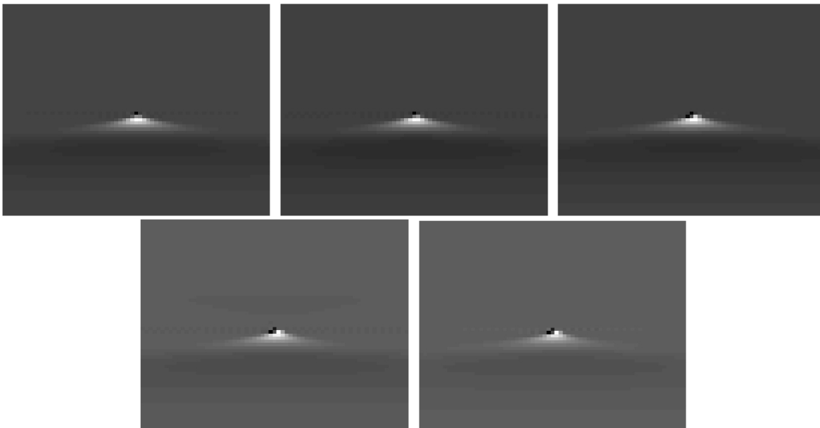
FIGURE 8. A possible approximation for the solution of minimal uncertainty for the scale-shear and scale-translations uncertainty that is admissible in the sense that it minimizes the admissibility condition integral. We provide this function for several values of the weight factor \alpha : \alpha = 0.1 (top left), \alpha = 1 (top middle), \alpha = 10 (top right), \alpha = 100 (bottom left) and \alpha = 10^6 (bottom right).
