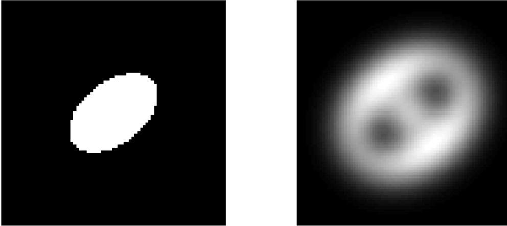
FIGURE 4. Sheared circle f_{0.5} (left) and \mathbb{T}_{(\psi_2,1,0)} (right, "wrong" shear factor).
