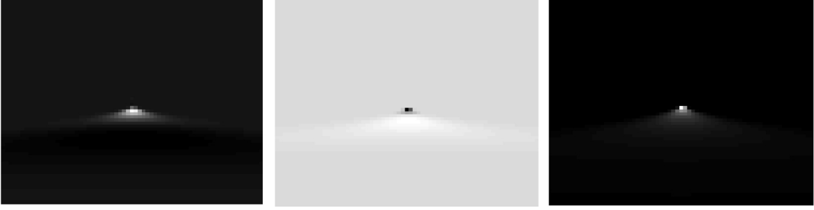
FIGURE 6. A possible solution for minimal uncertainty for the scale-shear and scale-translations uncertainty. The minimizer shown here is given by: \psi(x, y) = e^{-\frac{1}{2}(\frac{x}{y^2})^2} y^{-\frac{3}{2}+2i\mu_a} . On the left we see the real value of the function, at the middle its imaginary value and on the right its absolute value.
