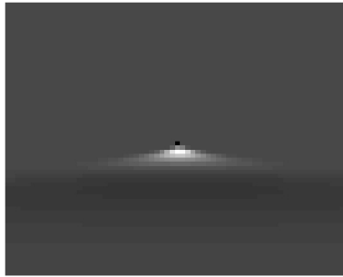
FIGURE 7. Original minimizer
