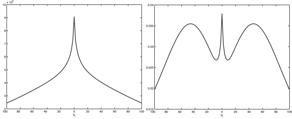
FIGURE 2 \int_{\mathbb{R}} |\hat{F}_{\theta, p_l}(p_h)|(1 + |p_h|)^{0.5}/(1 + |p_l|)^{0.5} dp_h , left: \theta = -2.642 , right: \theta = 1.758 .
