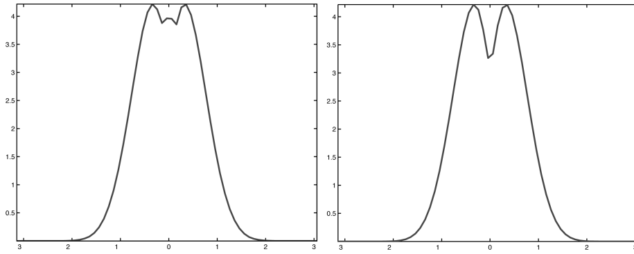
FIGURE 4 Maximum plot for all \theta \in [-\pi, \pi] ; left: \max_{p_l} \int_{\mathbb{R}} |\hat{F}_{\theta, p_l}(p_h)|(1 + |p_h|)^{0.5}/(1 + |p_l|)^{0.5} dp_h , right: \max_{p_h} \int_{\mathbb{R}} |\hat{F}_{\theta, p_l}(p_h)|(1 + |p_h|)^{0.5}/(1 + |p_l|)^{0.5} dp_l .
