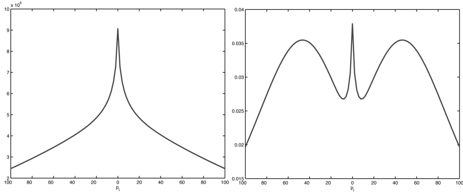
FIGURE 3 \int_{\mathbb{R}} |\hat{F}_{\theta, p_l}(p_h)|(1 + |p_h|)^{0.5}/(1 + |p_l|)^{0.5} dp_l , left: \theta = -2.642 , right: \theta = 1.758 .
